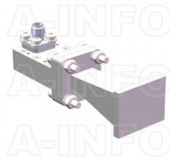
LB-42-10-C-3.5FSPO Standard Gain Horn Antenna 18-26.5GHz 10dB Gain 3.5mm Female
