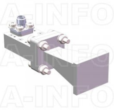
LB-42-10-C-KFSPO Standard Gain Horn Antenna 18-26.5GHz 10dB Gain 2.92mm Female
